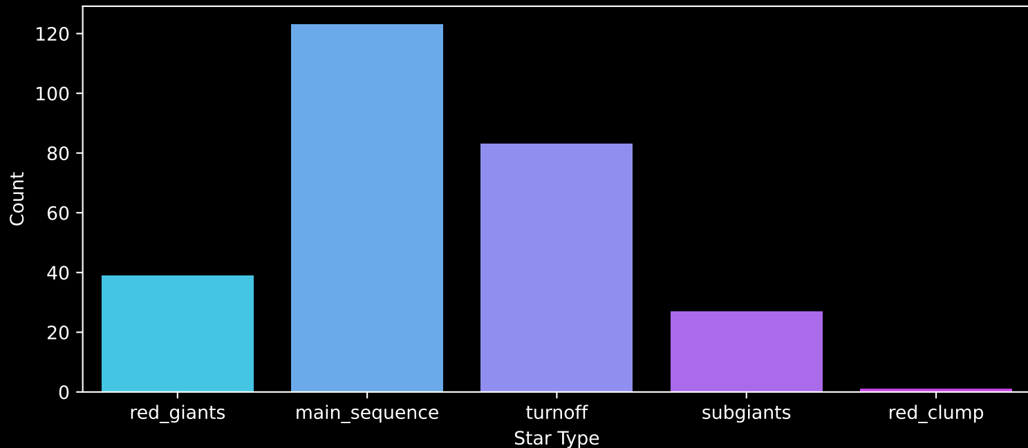
GALAH DR4 Field: [1467] Count plot of Star Type
