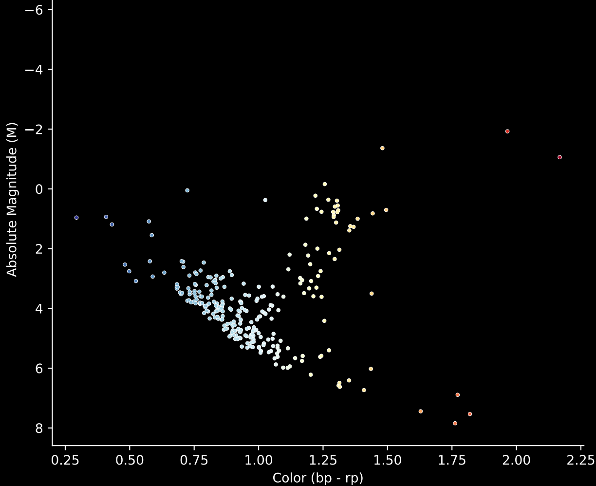
GALAH DR4 Field [1467] Stars (n= 273) Hertzsprung-Russel Diagram
