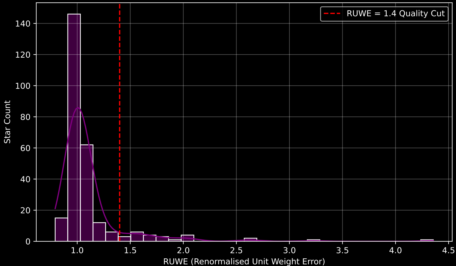
GALAH DR4 Field [1467] RUWE Distribution (n= 266)
