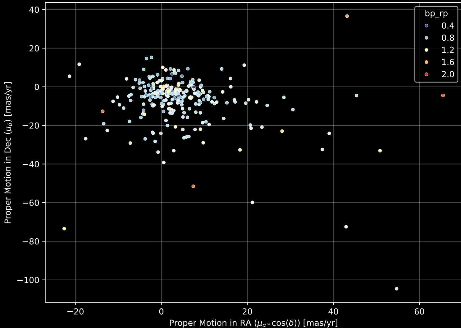
GALAH DR4 Field: [1467] Proper Motion Diagram (n= 273)
