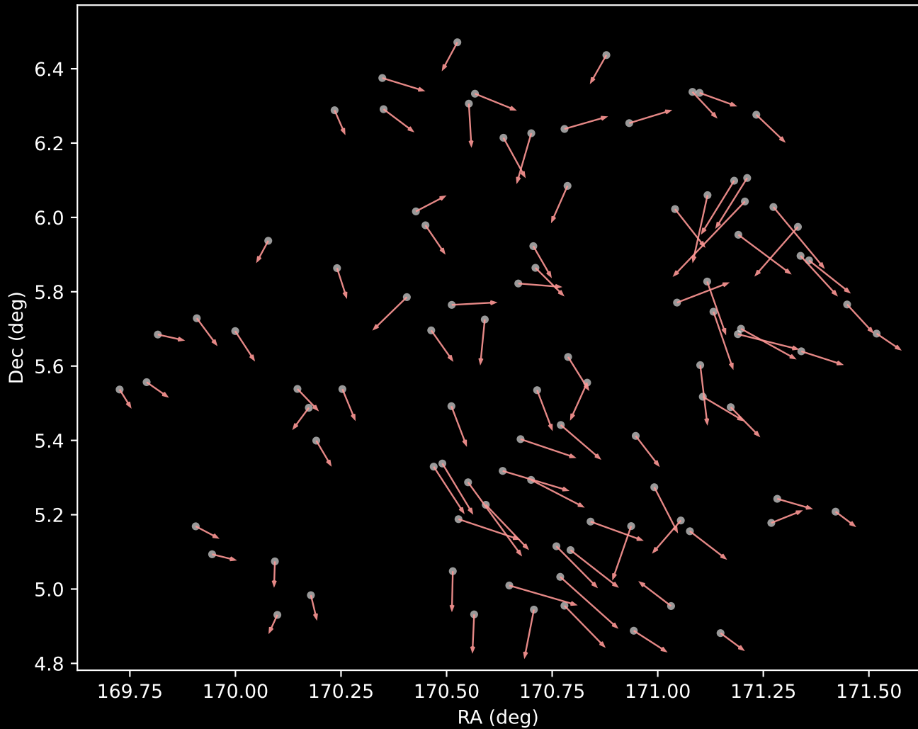
GALAH DR4 Cluster 7 Proper Motion Vectors (n=94)
